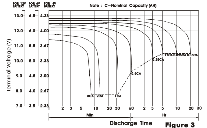
Figure 3. BP BATTERY DISCHARGE CHARACTERISTICS (25°C/77°F)
